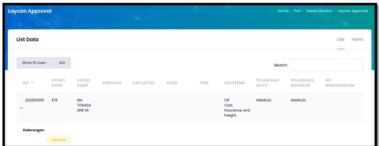
Gambar 10 approve laycan
